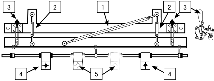
Big Gripper – Top View
